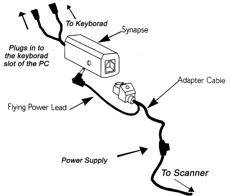
Figure "A" - Synapse and Adapter cable
